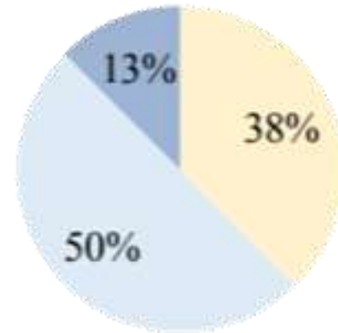
LaMDA (137B)
