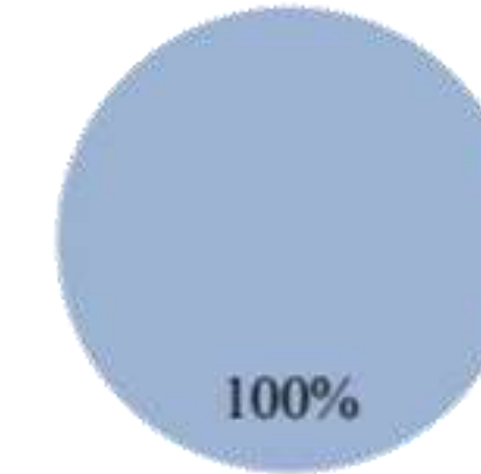
AlphaCode (41B)
