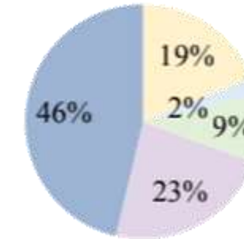
CodeGen (16B)
