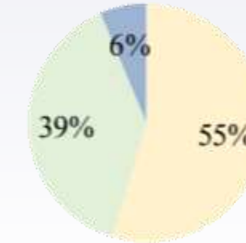
Chinchilla (70B)
