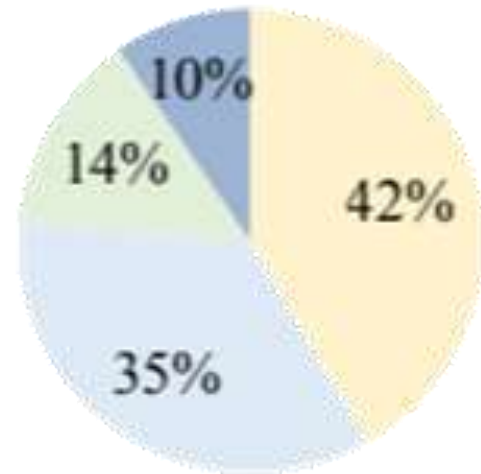
PaLM (540B)
