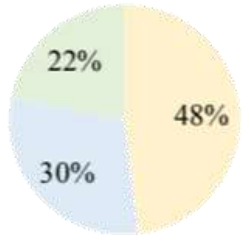
GLaM (1200B)
