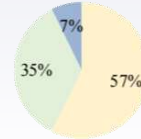
Gopher (280B)
