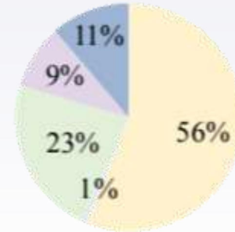
MT-NLG (530B)
